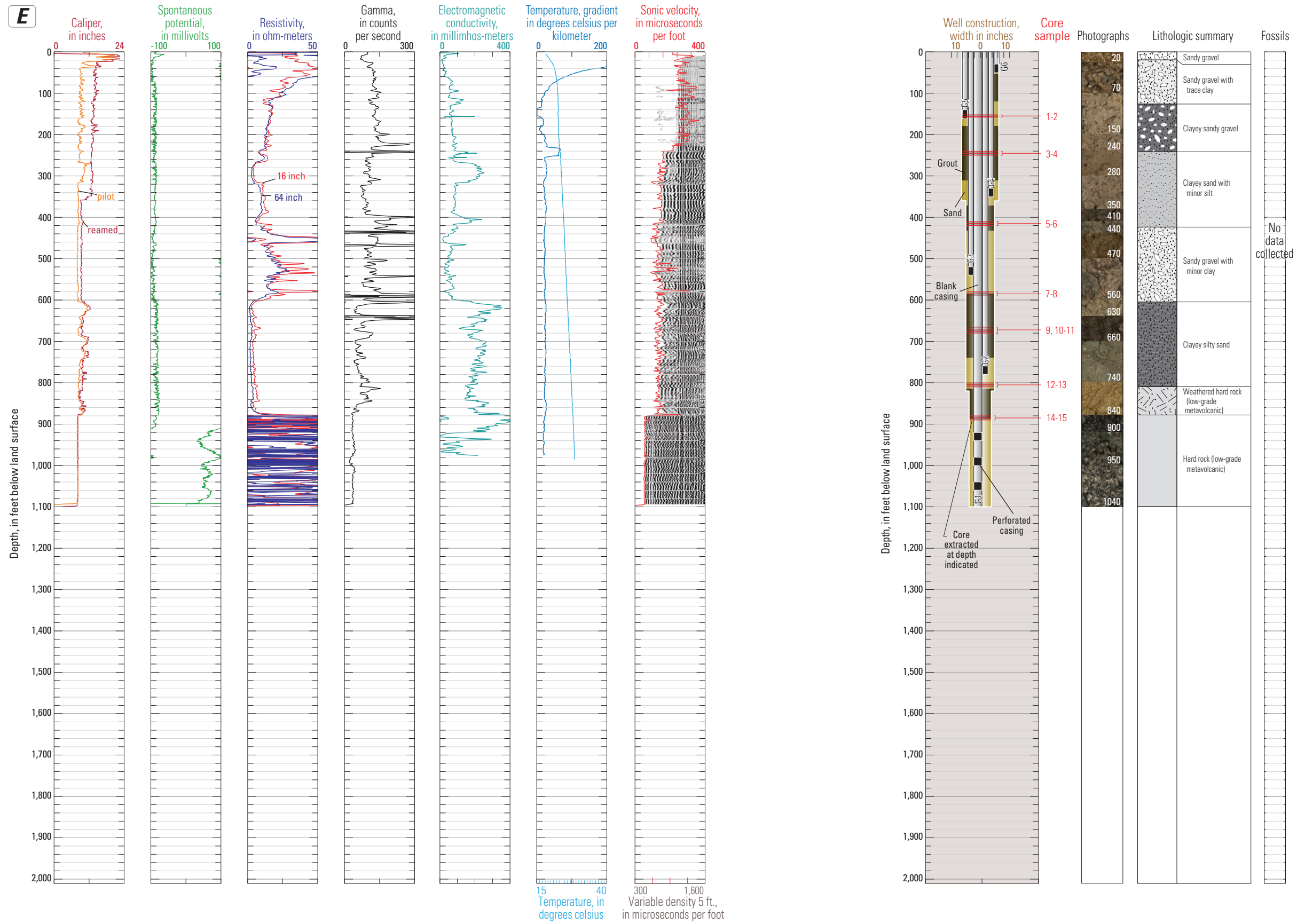
Figure 19E. Well-construction diagrams, generalized lithologic descriptions, and geophysical-log data for caliper, spontaneous potential, resistivity, natural gamma, electromagnetic conductivity, temperature, and sonic logs collected from 16 USGS multiple-depth, monitoring-well sites in San Diego County, California, 1995, 2003–2017: (A) SDCD; (B) SDSY; (C) SDLH; (D) SDAQ; (E) SDCP ; (F) SDBP; (G) SDHF; (H) SDEP; (I) SDNB; (J) SDSW; (K) SDMC; (L) SDLD; (M) SDCC; (N) SDOR; (O) SDOT; and (P) SDBW.—Continued.
